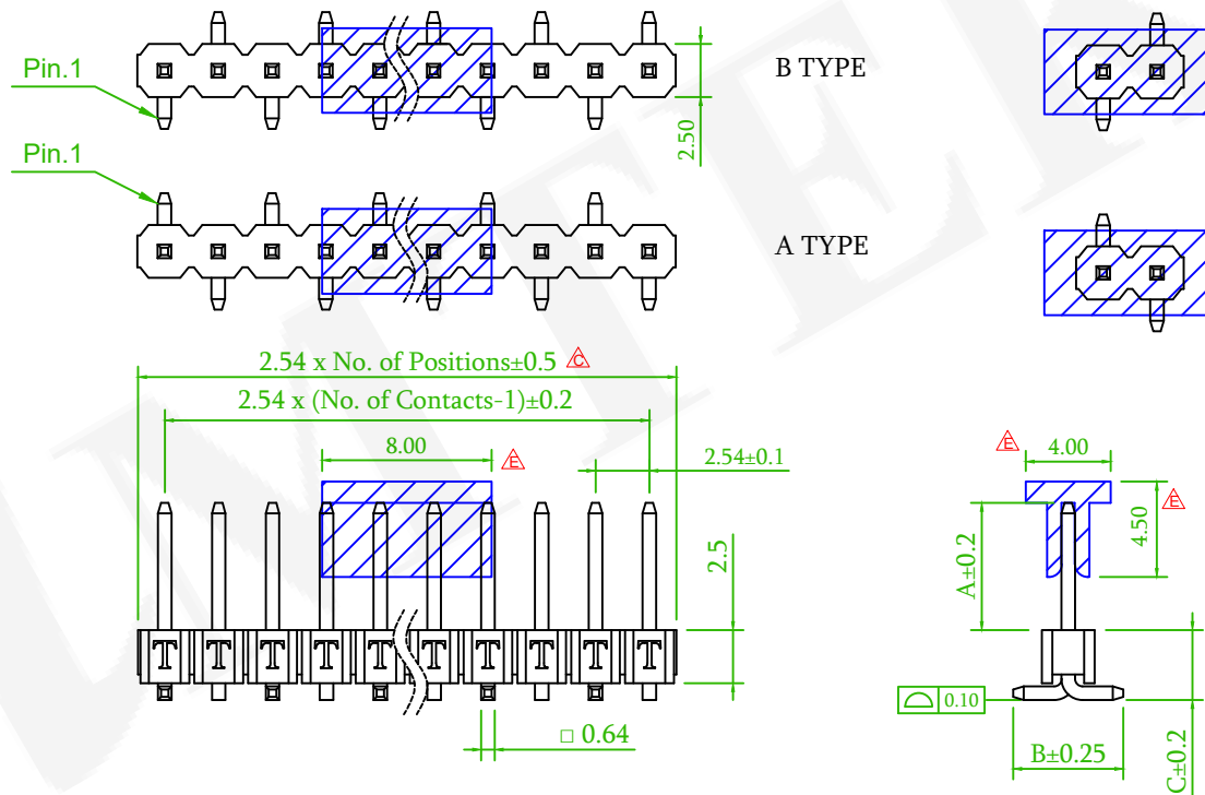
Old Part No. :PH1M25-1XX-U
