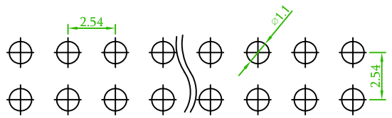
Recommended PCB Layout (PCB TOLERANCE ±0.1)
