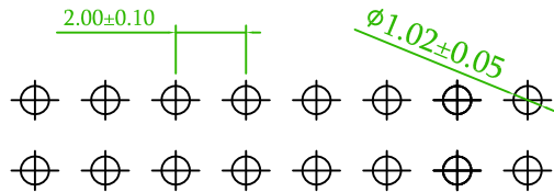
Recommended PCB Layout (PCB TOLERANCE ±0.05)
