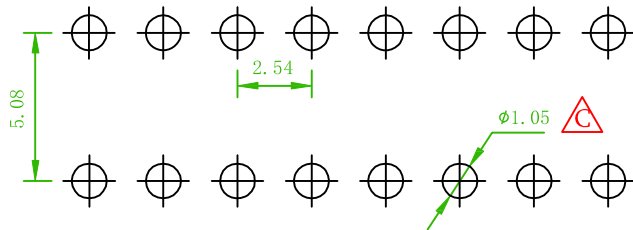
Recommended PCB Layout (PCB TOLERANCE ±0.1)
