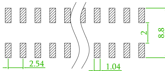
PCB LAYOUT TOLERANCE ±0.1
