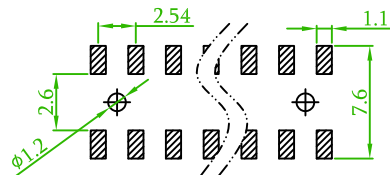
Recommended P.C.B Layout (PCB BOARD TOLERANCE±0.1)
