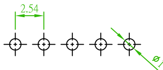
Recommended PCB Layout (PCB TOLERANCE ±0.1)
