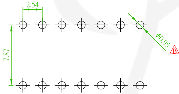
Recommended PCB Layout (PCB TOLERANCE ±0.05) \Delta B
