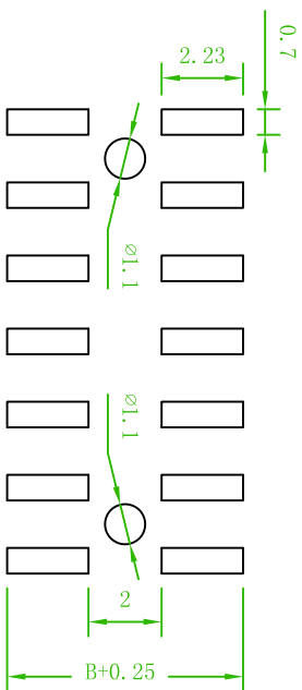
Recommended PCB Layout (PCB TOLERANCE±0.05)
